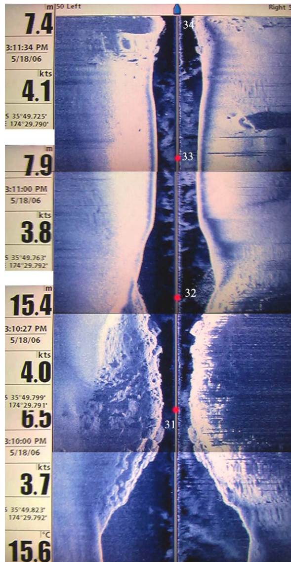
Figure 5. Representative sonar images. This image is a composite of a series of screen shots on a survey line from sonar points 31-34 (refer Map Section Map 1). This track runs from south to north just past the west end of Motukaroro Island. The distance from data point 31 to point 34 is 181 m.
