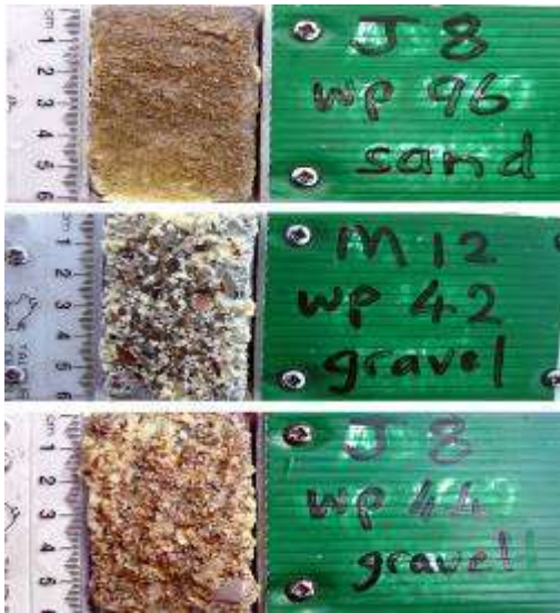
Figure 4 Example of rapid sediment samples
