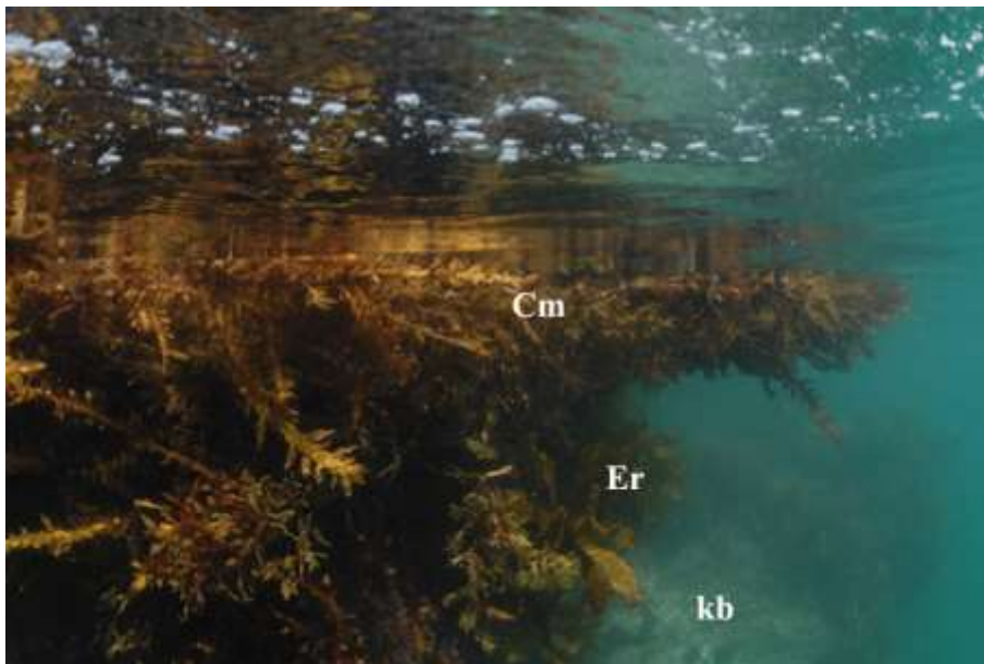
Figure 14 Shallow mixed weed habitat at Akeake Point (Profile 3) on the western shore of Urupukapuka Island. Carpophyllum maschalocarpum (Cm), Ecklonia radiata (Er), kina barren (kb)
