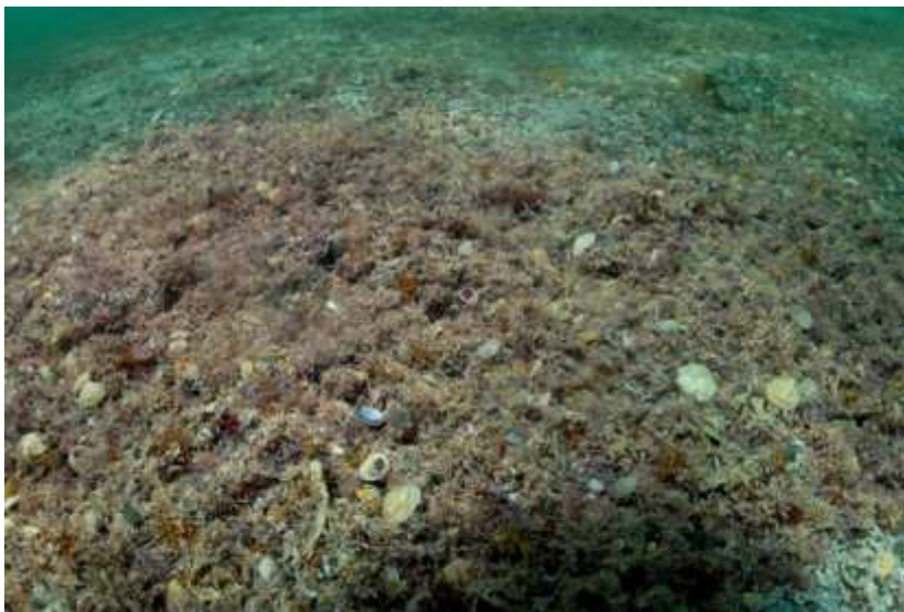
Figure 21 Algal turf habitat growing on a coarse sand, shell, and gravel substrate typical of the Okahu Channel bottom
