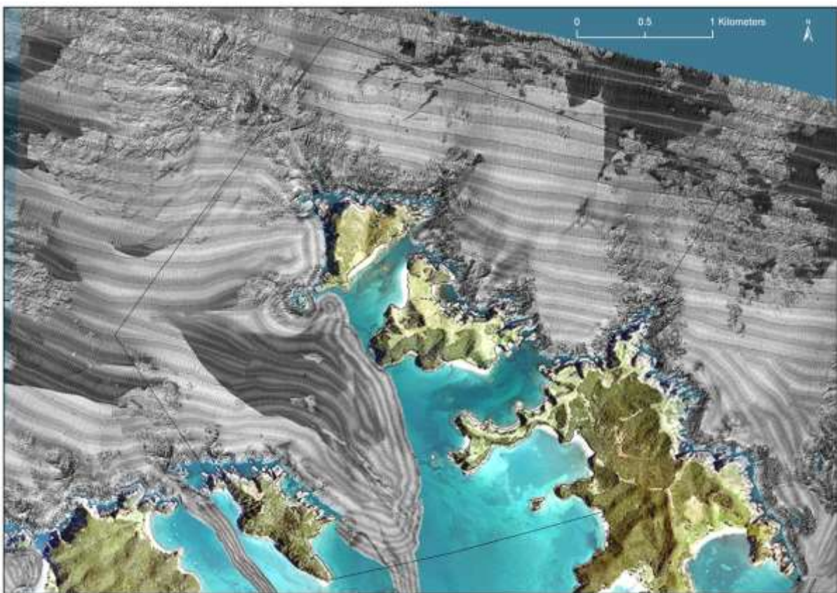
Figure 7 OS 20/20 multibeam backscatter layer displayed over a contour hillshade bathymetry layer. The thin black line depicts the mapping area.
